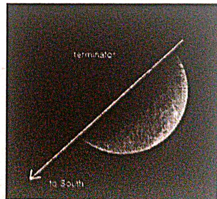
Figure 2: The line along the terminator when extended points to the South.
